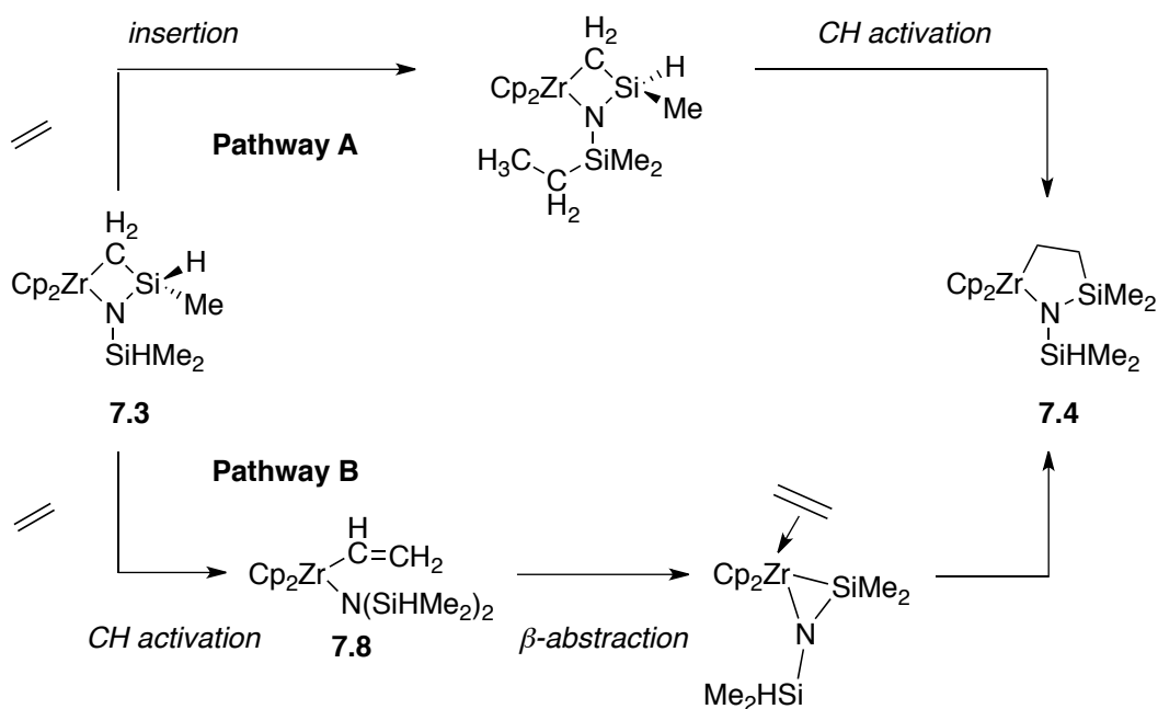
Scheme 7.2. Possible H 2 -free pathways for conversion of 7.3 to 7.4.
