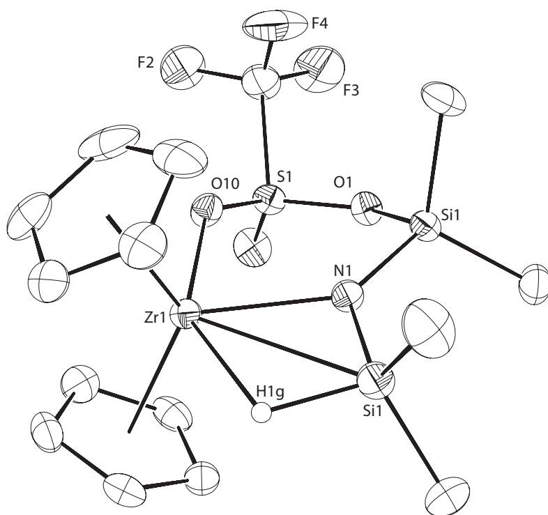
Figure 9.3. ORTEP diagram of [\text{Cp}_2\text{ZrN}(\text{SiHMe}_2)(\text{SiMe}_2-\mu-\kappa^2\text{-OTf})][\text{HB}(\text{C}_6\text{F}_5)_3] ( [9.12][HB(C 6 F 5 ) 3 ] ). The cationic portion of the structure is illustrated, and only the bridging hydrogen atom is plotted. All other hydrogen atoms, the HB(C 6 F 5 ) 3 counterion, and a disordered C 6 H 5 Br molecule are not included for clarity.
