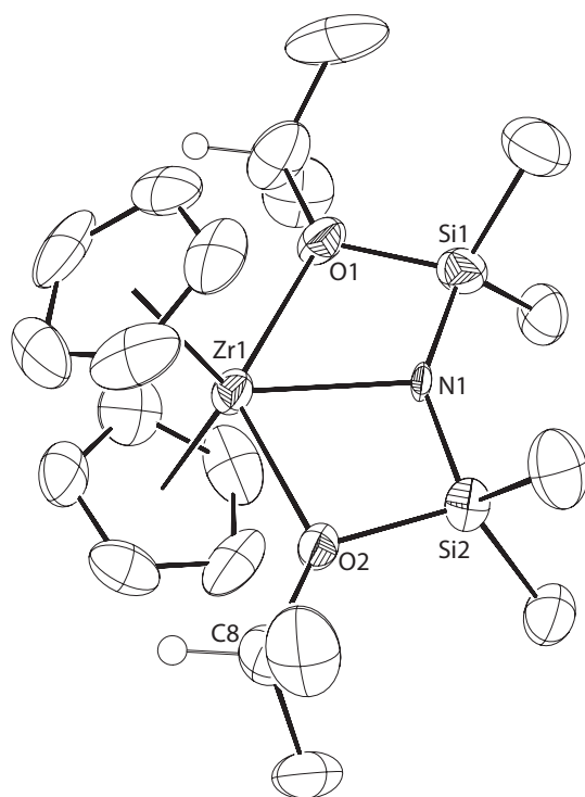
Figure 9.3. ORTEP diagram of the cationic portion of [9.22] + with ellipsoids plotted at 50% probability. The HB(C 6 F 5 ) 3 and a CH 2 Cl 2 solvent molecule are not illustrated. The hydrogen on the C 5 H 5 and methyl groups are not shown for clarity. Significant interatomic distances (Å): Zr1-N1, 2.121(4); Zr1-O1, 2.385(4); Zr1-O2, 2.333(3); N1-Si1, 1.642(4); N1-Si2, 1.712(4); Si1-O1, 1.711(4); Si2-O2, 1.699(4). Selected interatomic angles (°): Zr1-N1-Si1,
